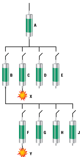
In a selective system: For a fault at "X" only fuse "C" will open. For a fault at "Y" only fuse "F" will open.
