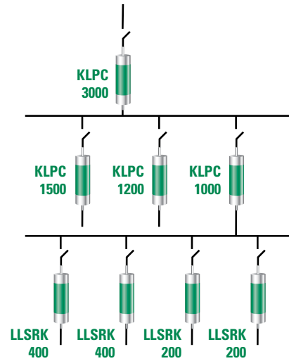
Figure 16 A Coordinated (selective) Fused System
